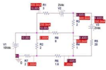
Figure S2.70: Bridge Circuit with Current source for Problem 2.70.
