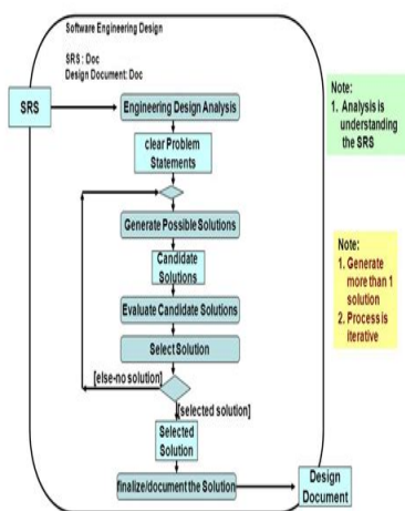
Software Engineering Design (in Activity Diagram)
