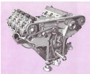
Fig. 9 - Valve Train Drive
