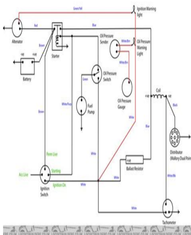
Rover V8 wiring diagram
