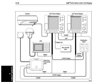
Figure 8-15: Integrated System with Repetitive Display and NMEA Instruments
