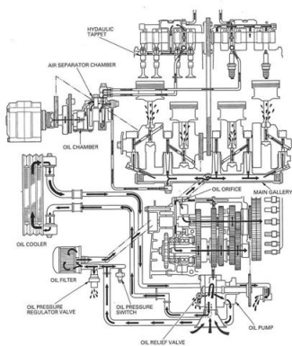
LUBRICATION SYSTEM LUBRICATION SYSTEM DIAGRAM
