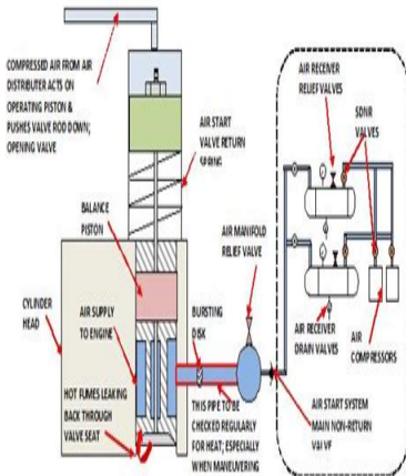
TYPICAL AIR START SYSTEM ON A MODERN TWO-STROKE MARINE DIESEL ENGINES SHOWING LEAKING AIR START VALVE & SAFETY DEVICES AGAINST EXPLOSION
