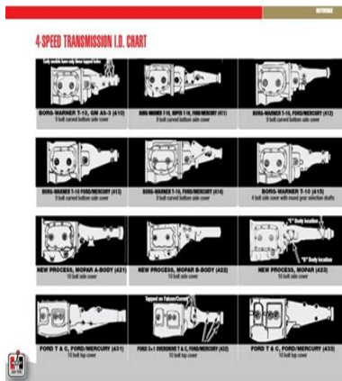
4 Speed Manual Transmission ID Chart
