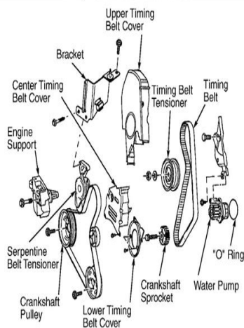
2009 Volkswagen New Beetle GL Fig. 4: Exploded View Of Timing Belt & Components (AEG, AVH, AZG, BDC & BEV Engine Codes) Courtesy of VOLKSWAGEN UNITED STATES, INC.
