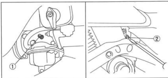
Fig. 4-9 (1) Throttle stop screw (2) Air screw
