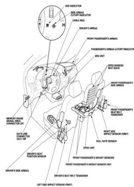
Fig. 1: Identifying SRS Components Location (1 OF 2) Courtesy of AMERICAN HONDA MOTOR CO., INC.
