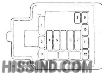
UNDER-HOOD FUSE BOX
