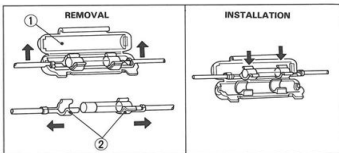
Fig. 4-22 (1) Fuse holder (2) Clips
