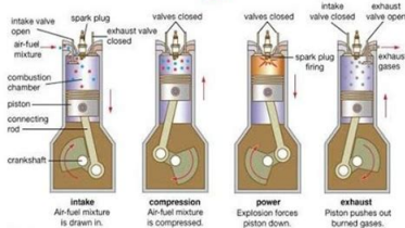
Four Stroke
