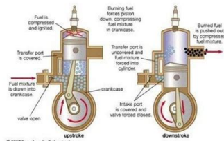
Two Stroke
