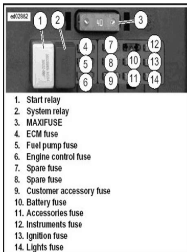
Figure 4-24. Fuses and Relays
